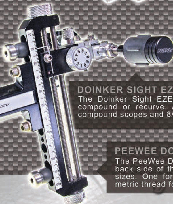
EZE Doinker Sight EZE, 0.9oz 10/32 Thread (F) Compound or 8/32 (F) Recurve
